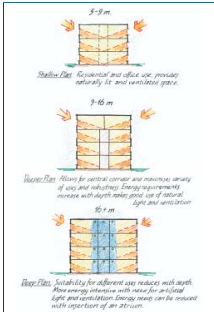
The relationship between plan form, ventilation and natural light
